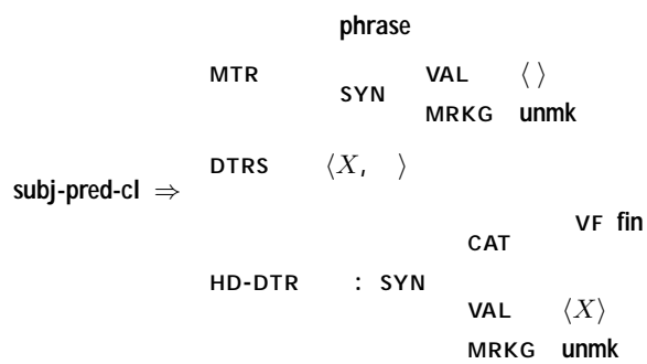
FIGURE 3 The (Combinatoric) Subject-Predicate Construction (Sag this volume, (110))
