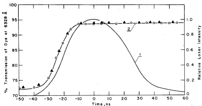
Fig. 5. Transmission of H 2 Pc at 6328 Å versus time. Plot 1—ruby laser pulse shape; ○—experimental data of [7]; △—calculated points with proposed model and Table I parameters. Laser peak intensity: 2.6
